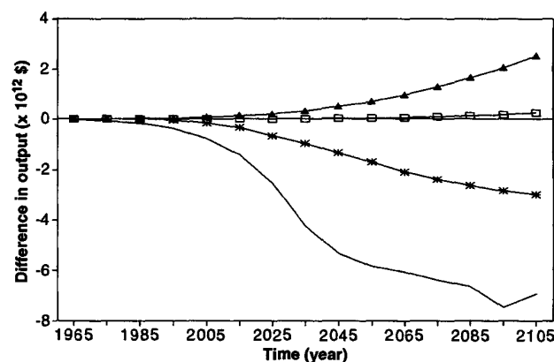
Fig. 5. Impact of policies on global output. The DICE model calculates the difference in economic welfare between a policy and a no-controls approach. The optimal policy ( \square ) leads to slightly lower output in the first few decades, then raises output modestly after 2025. Geoengineering ( \blacktriangle ) produces major benefits, whereas emissions stabilization (*) and climate stabilization (—) are projected to be worse than inaction.
