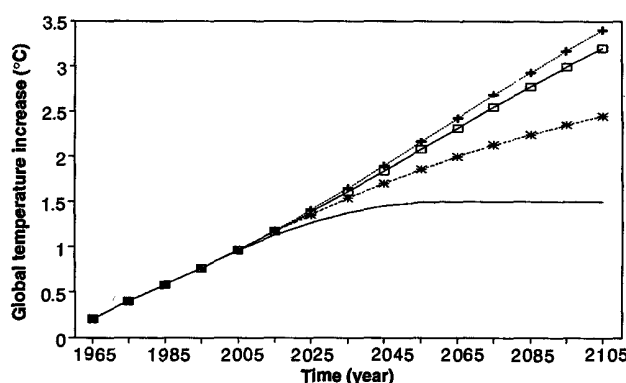
Fig. 3. Projected global mean temperature. According to the DICE model, global mean temperature with no controls (+) is projected to increase 3°C above 1900 levels by 2085. The optimal policy ( \square ) and emissions stabilization (*) would involve only a small reduction in global warming. The maximum feasible policy is climate stabilization (—), which shows significant warming because of the commitment in the current buildup of GHGs.
