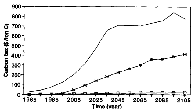
Fig. 4. Carbon taxes in different policies to reduce GHGs. Carbon taxes are a good index of the stringency of policies to slow global warming. A carbon tax would penalize production and consumption of fossil fuels and CFCs and encourage afforestation. Calculations indicate that the optimal carbon tax ( \square ) rises from around $5 to about $20 per ton of carbon in 2100. Emissions stabilization (*) and climate stabilization (—) imply sharply rising carbon taxes that would raise coal prices severalfold. Carbon tax given in 1989 U.S. dollars.
