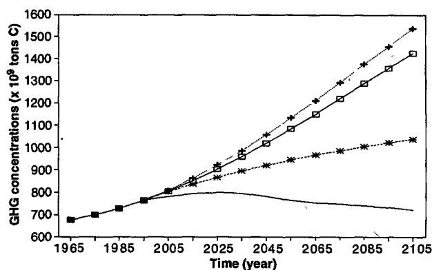
Fig. 2. Greenhouse-gas concentrations. Concentrations of GHGs (including \text{CO}_2 and CFCs, in \text{CO}_2 -equivalent basis) are estimated to double from pre-industrial levels around 2050 for the uncontrolled path (+). The optimal path ( \square ) shows a small reduction in concentrations, whereas emissions stabilization (*) leads to continued increases. Climate stabilization (—) would require declining concentrations.
