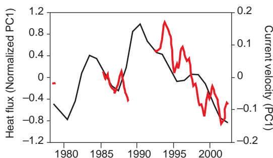
Spinning down. When the North Atlantic's subpolar gyre began losing less heat (black) in the mid-1990s, it slowed (red).
