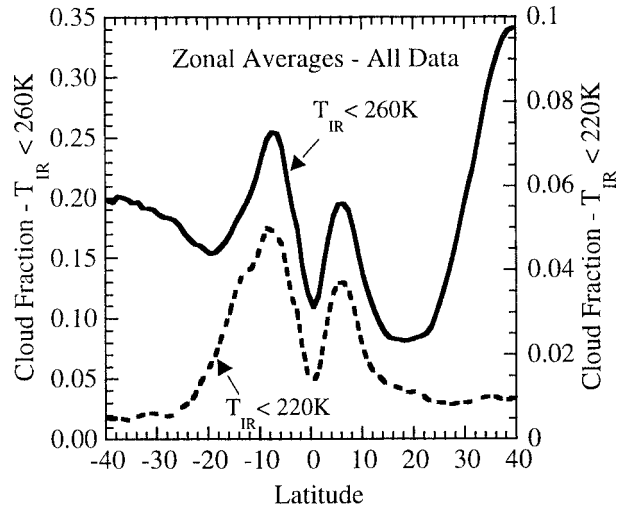
FIG. 4. Zonally averaged T_{11} < 260 K cloud fractions for the oceanic areas in the region 130^{\circ}\text{E} – 170^{\circ}\text{W} for all days with data in the period 1 Jan 1998–31 Aug 1999.
